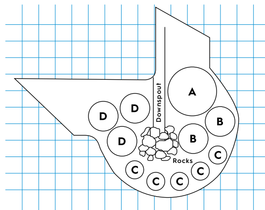
LAYOUT DIAGRAM (each square = 1 foot)
