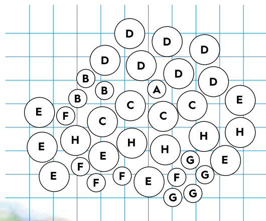
LAYOUT DIAGRAM (each square = 1 foot)
