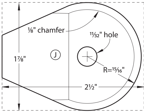
HITCH FULL-SIZE PATTERN (Top view)
