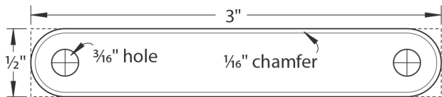
Ⓡ BRACKET FULL-SIZE PATTERN
