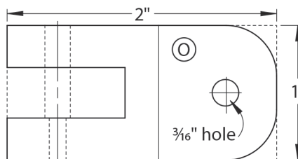
PIVOT BRACKET SIDE-VIEW FULL-SIZE PATTERN
