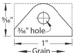
Ⓡ BRACKET FULL-SIZE PATTERN
