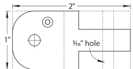
PIVOT BRACKET TOP-VIEW FULL-SIZE PATTERN
