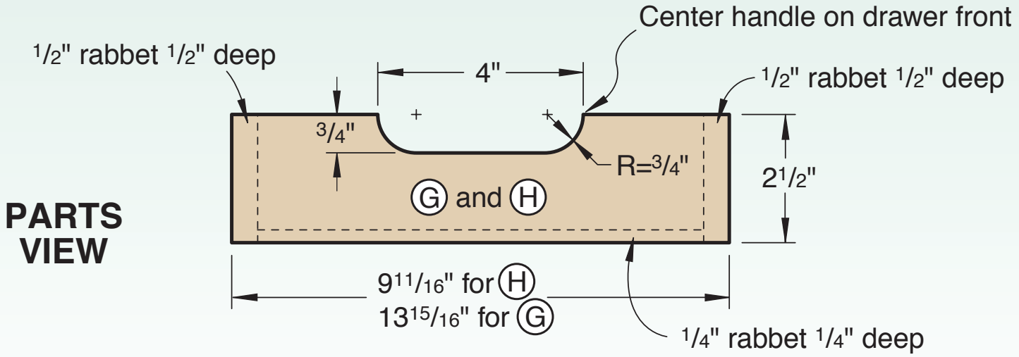
DRAWER FRONTS
